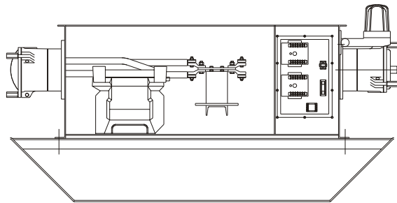
15 kV, 500 A SPLITTER BOX
